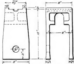
Figs. 1755-1756. Driving Box Saddle for Consolidation (2-8-0) Locomotive. American Locomotive Co.
